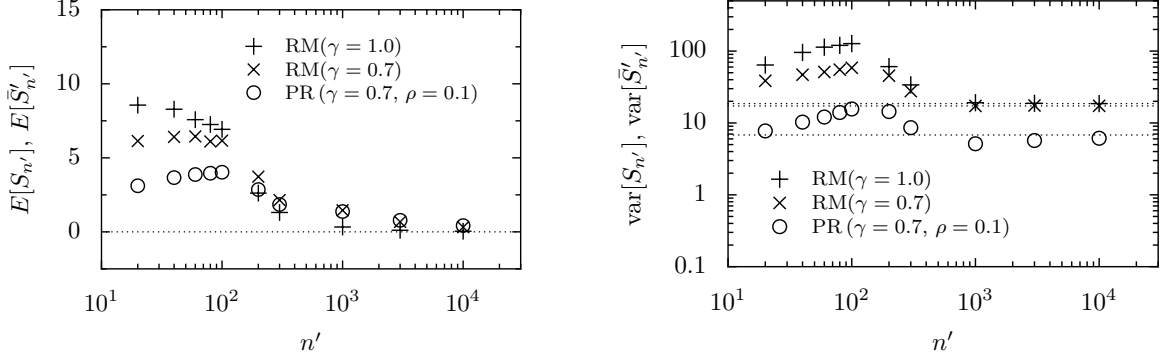
Figure 11: NCM, polynomial SR ( \eta = 2.0 , \lambda = 0.05 ), and exponential twisting .– Empirical mean values and variances of the rescaled quantities S_{n'} = \sqrt{n'}^\gamma (s_{n'} - s^*) and \bar{S}_{n'} = \sqrt{\rho n'} (\bar{s}_{n'} - s^*) , corresponding to the histograms from Fig. 11. For large enough n' , the variances converge to the values predicted by Theorems 3.13/3.16 (dotted lines, obtained by using the estimators from Th. 3.18).
