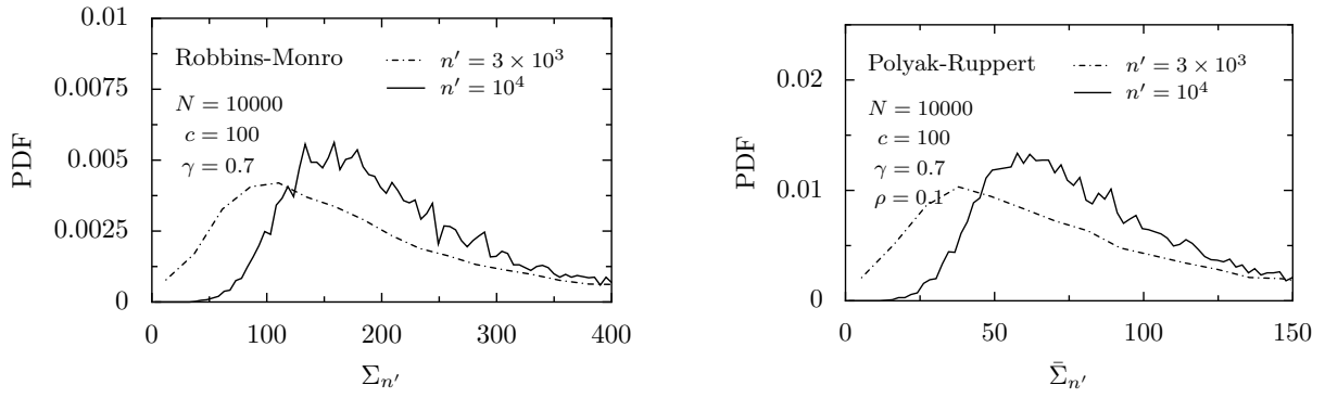
Figure 8: NCM model and polynomial loss function (without importance sampling). — Illustration of Theorem 3.18: Histogram of the variances \Sigma_{n'} and \bar{\Sigma}_{n'} , using the estimators from Theorem 3.18, respectively. Importance sampling yields considerable variance reduction, cf. Fig. 12 below.
