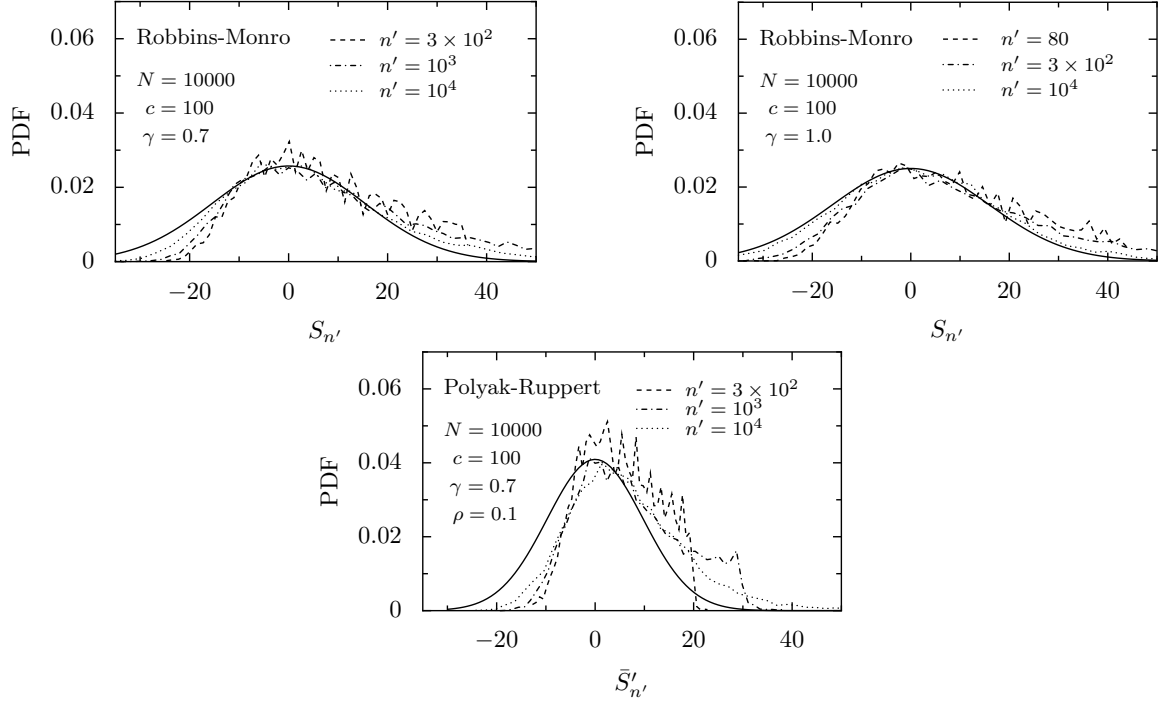
Figure 7: NCM and polynomial SR with \eta = 2.0 and \lambda = 0.05 (without importance sampling). —Asymptotically, the rescaled quantities S_{n'} = \sqrt{n'\gamma}(s_{n'} - s^*) and \bar{S}'_{n'} = \sqrt{\rho n'}(\bar{s}'_{n'} - s^*) approach Gaussian distributions (cf. Theorems 3.13 and 3.16). For large n' , the numerical results approach the theoretical prediction (solid lines, obtained by using the estimators from Th. 3.18), but again convergence is very slow.
