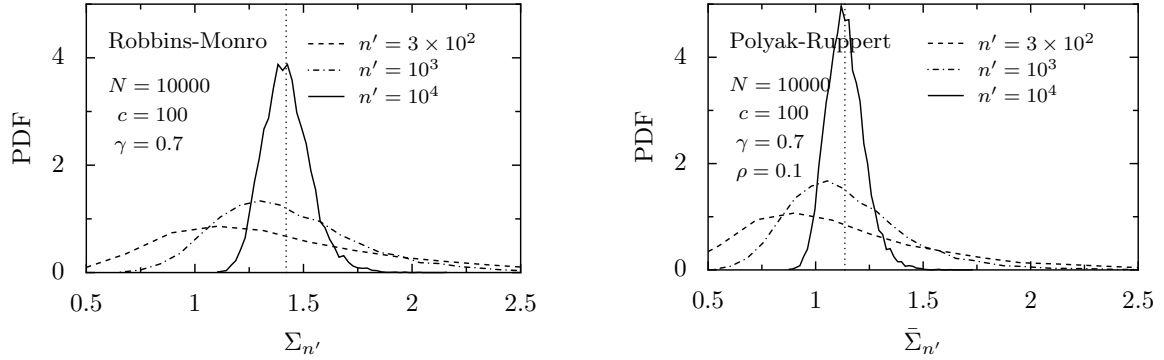
Figure 3: Gaussian loss distribution and exponential loss function. – Illustration of Theorem 3.18: Histogram of the variances \Sigma_{n'} and \bar{\Sigma}_{n'} , using the estimators from Theorem 3.18, respectively. The vertical lines indicate the exact results.
