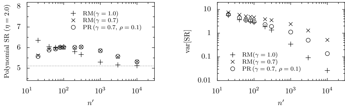
Figure 6: NCM and polynomial SR with \lambda = 0.05 (without importance sampling). – Left: The different algorithms converge slowly to the same SR value s^* = 5.11 (determined from IS). Right: Sample variances of the SR estimates in the left diagram. As evident from the diagrams, without IS the convergence is very slow. The results are qualitatively similar to those obtained for the Frechet type heavy tail distribution, cf. Fig. 5.
