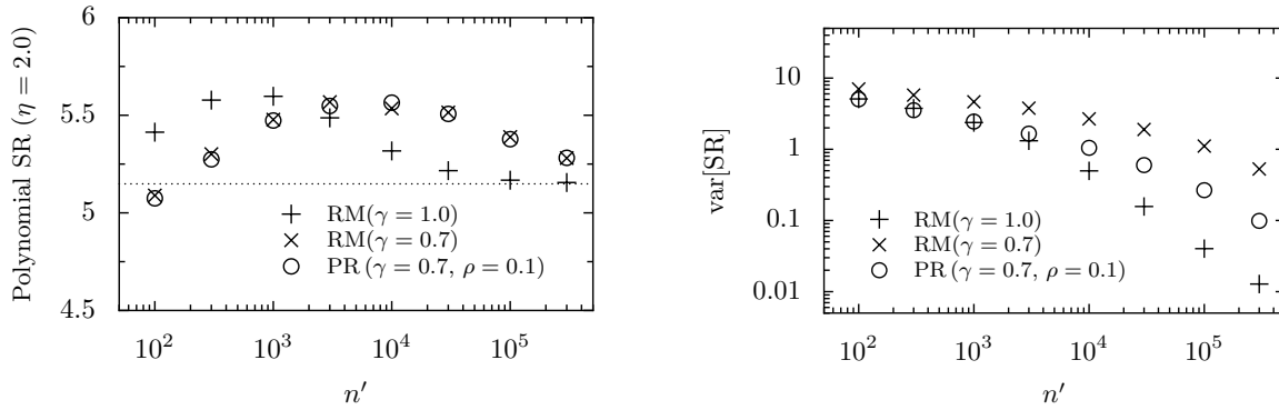
Figure 5: Heavy-tailed Frechet type loss distribution (25) and (piecewise) polynomial SR with \lambda = 0.05 . – Left: The different algorithms converge to the same SR value s^* = 5.1486 . Right: Sample variance of the SR estimates in the left diagram. The convergence is considerably slower than in the case of light-tailed Gaussian loss distributions, cf. Fig. 4.
