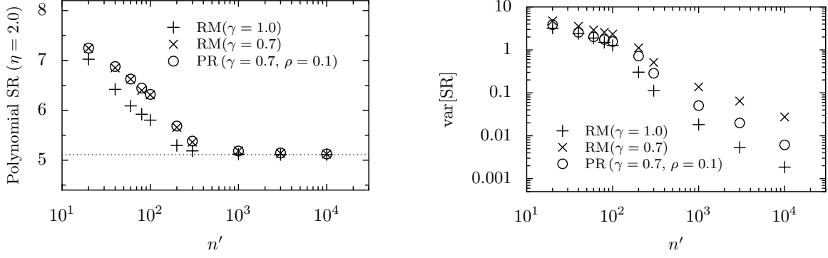
Figure 9: NCM, polynomial SR ( \eta = 2.0 , \lambda = 0.05 ), and exponential twisting .– Left: The different algorithms converge to the same SR value s^* = 5.11 . Right: Sample variances of the SR estimates in the right diagram. Convergence has considerably improved, cf. Fig. 6.
