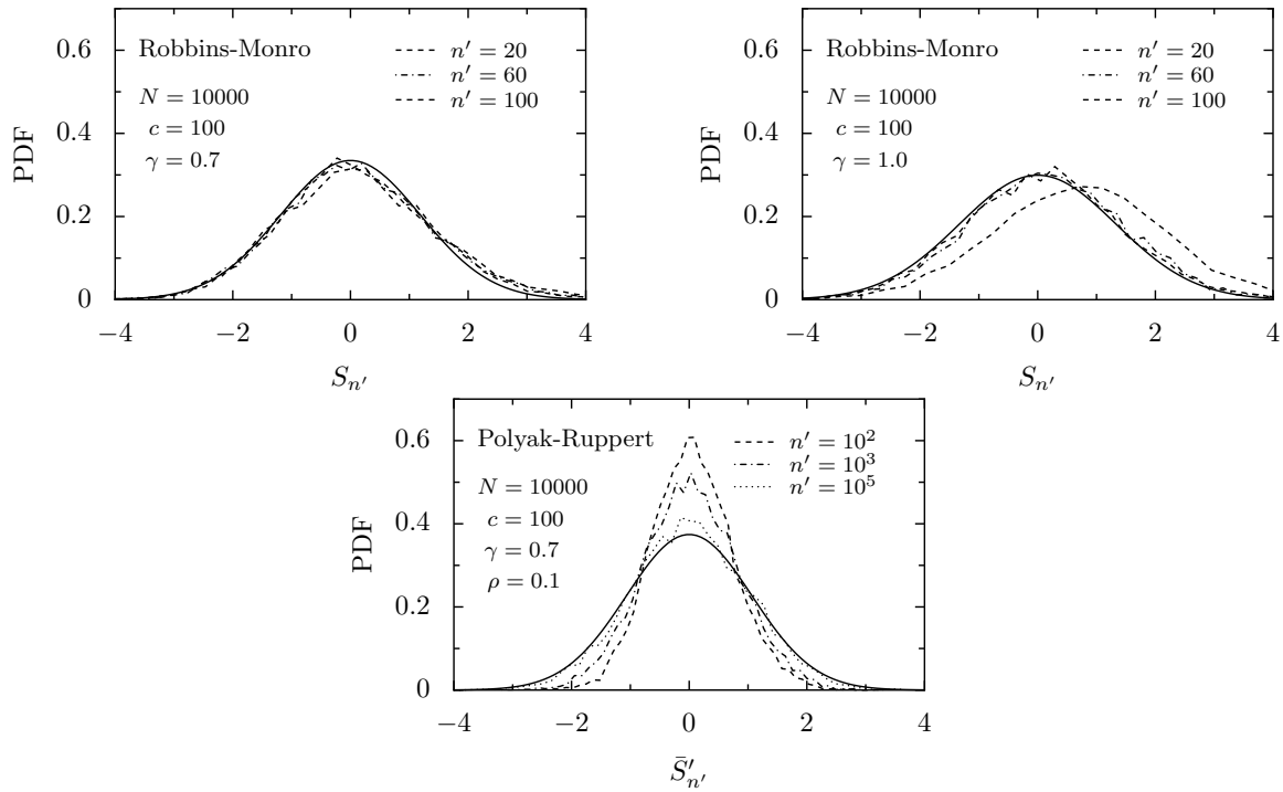
Figure 1: Gaussian loss distribution and exponential loss function. – Asymptotically, the rescaled quantities S_{n'} = \sqrt{n'\gamma}(s_{n'} - s^*) and \bar{S}'_{n'} = \sqrt{\rho n'}(\bar{s}'_{n'} - s^*) approach Gaussian distributions (cf. Theorems 3.13 and 3.16). The numerical results agree with the theoretical prediction (solid lines).
