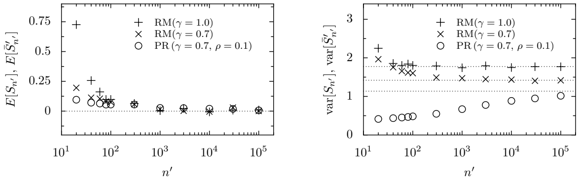
Figure 2: Gaussian loss distribution and exponential loss function. – Empirical mean values and variances of the rescaled quantities S_{n'} = \sqrt{n'}^\gamma (s_{n'} - s^*) and \bar{S}_{n'} = \sqrt{\rho n'} (\bar{s}_{n'} - s^*) , corresponding to the histograms from Fig. 1. For large enough n' , the variances converge to the values predicted by Theorems 3.13/3.16 (dotted lines).
