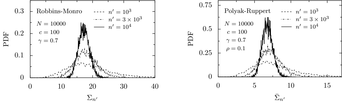
Figure 12: NCM, polynomial SR ( \eta = 2.0 , \lambda = 0.05 ), and exponential twisting .– Illustration of Theorem 3.18: Histogram of the variances \Sigma_{n'} and \bar{\Sigma}_{n'} , using the estimators from Theorem 3.18, respectively. Importance sampling has led to a considerable variance reduction, cf. Fig. 8 above.
