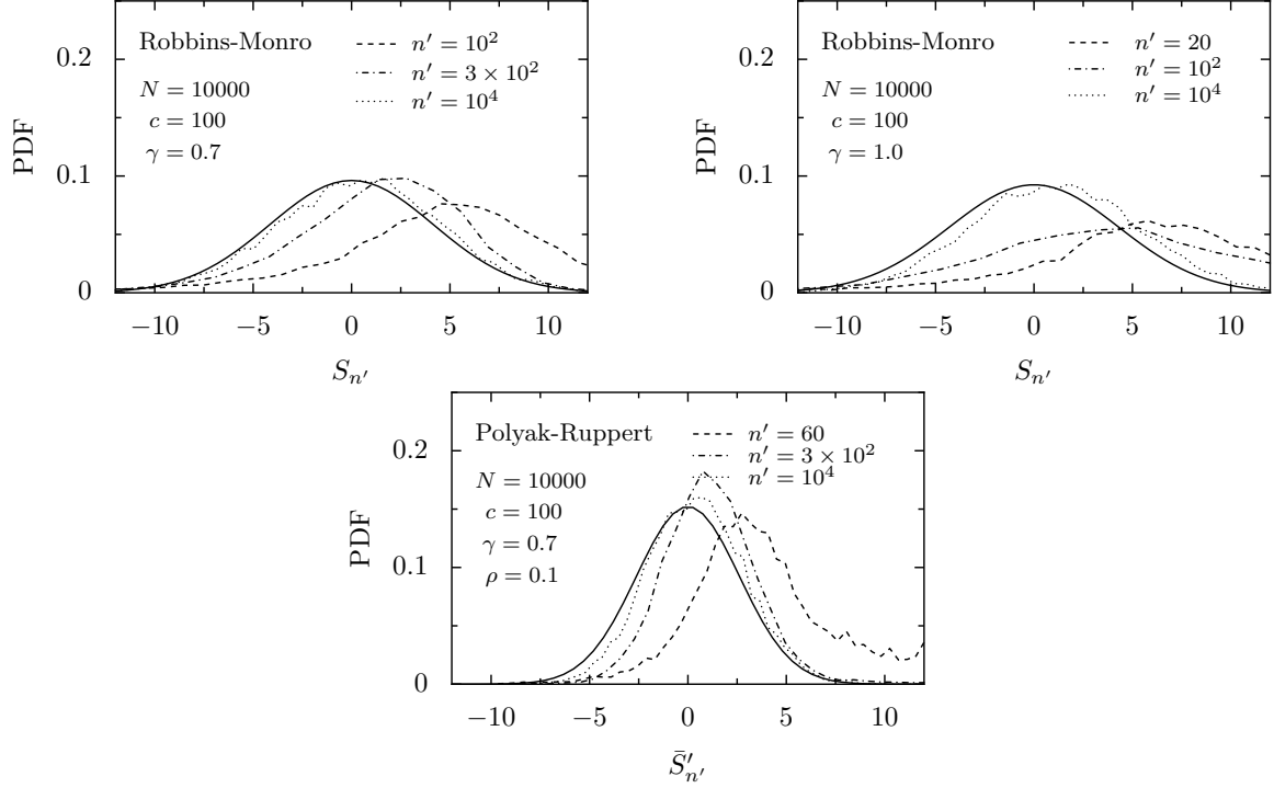
Figure 10: NCM, polynomial SR ( \eta = 2.0 , \lambda = 0.05 ), and exponential twisting .– Asymptotically, the rescaled quantities S_{n'} = \sqrt{n'^\gamma}(s_{n'} - s^*) and \bar{S}_{n'} = \sqrt{\rho n'}(\bar{s}_{n'} - s^*) approach Gaussian distributions (cf. Theorems 3.13 and 3.16). For large n' , the numerical results approach the theoretical prediction (solid lines, obtained by using the estimators from Theorem 3.18).
